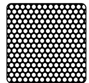
Protec's mesh is thermally treated for increased strength and performance, made from a solid 1.7mm aluminium sheet with 2.0 mm holes, providing an improved open area of 40.3% and viewing angle of 135°.
